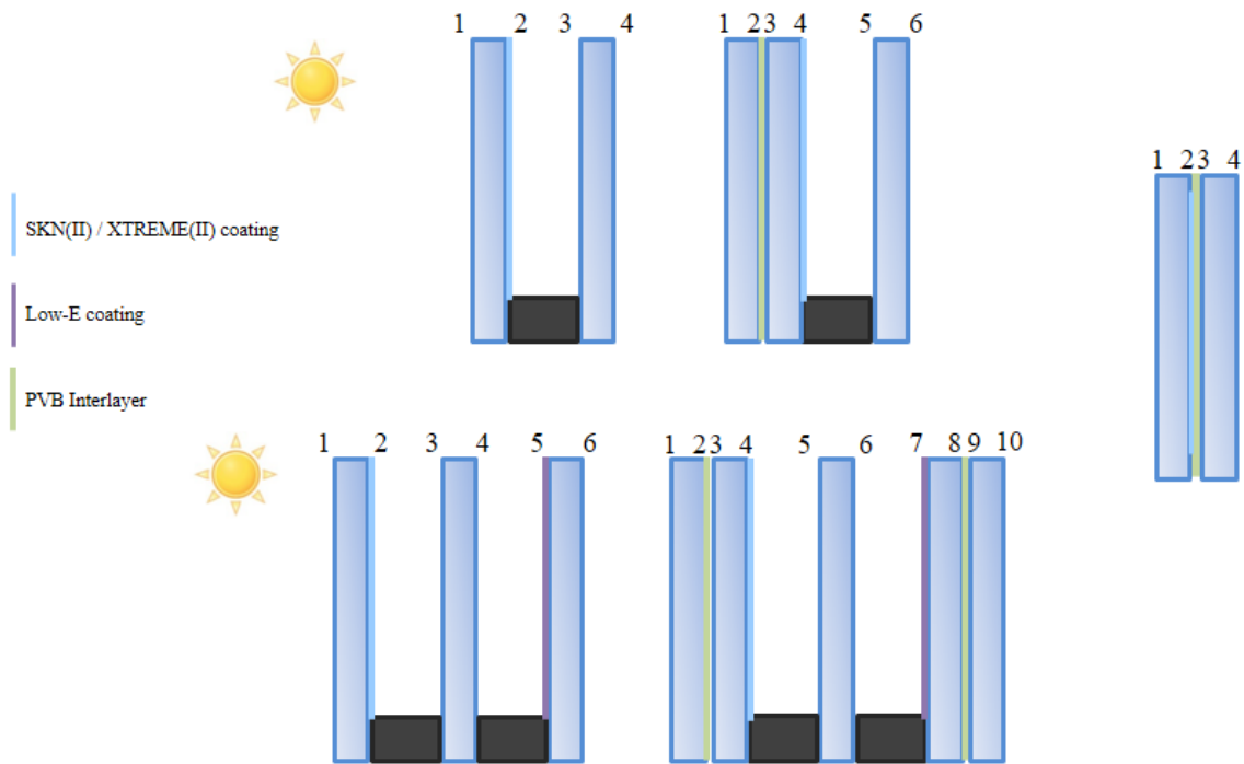
Figure 2: Possible configurations of use of COOL-LITE® SKN (II) / COOL-LITE® XTREME (II) In all cases, the coating must be edge deleted.
